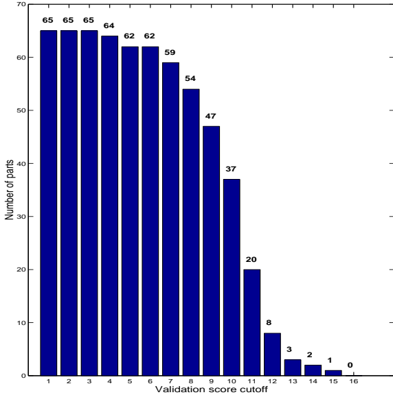
Fig. 3. Subjects validity
